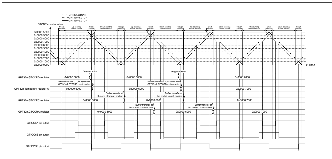
Figure 23.46 Example of Complementary PWM Mode 1 Operation (GTIOCnA pin = Low / GTIOCnB pin = High at GTCCRA register compare match during up-counting, GTIOCnA pin = High / GTIOCnB pin = Low at GTCCRA register compare match during down-counting, the dead time value is 0x0000 1000 and updating GTCCRD register in crest and trough sections) (n = 4, 7)
