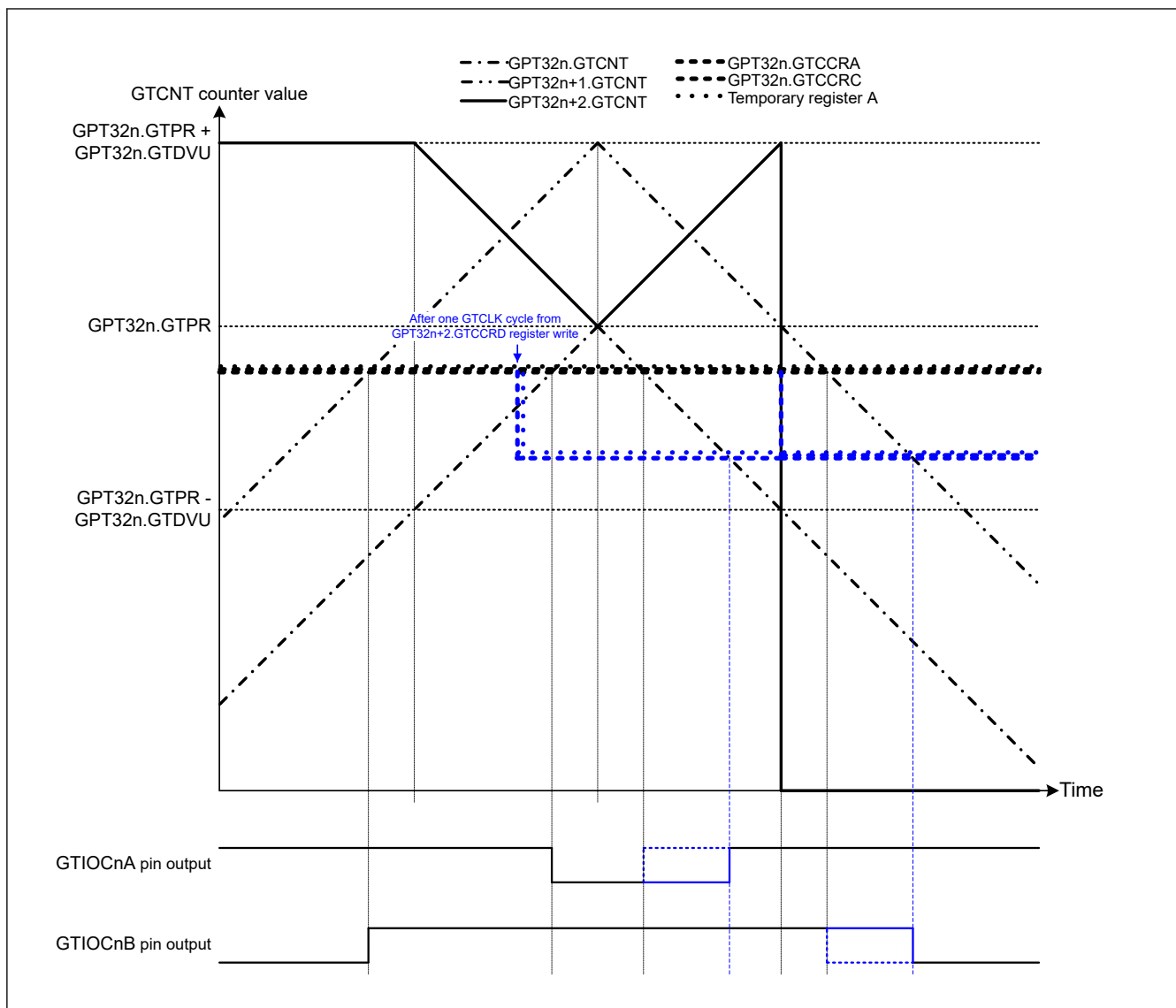
Figure 23.69 Example of Complementary PWM Mode 4 Single Buffer Operation (Up-Counting Crest Section) (Complementary PWM mode 4 single buffer operation, GTIOCnA pin = Low / GTIOCnB pin = High at GTCCRA register compare match during up-counting, GTIOCnA pin = High / GTIOCnB pin = Low at GTCCRA register compare match during down-counting, when a value is written to GTCCRD register during the up-counting dead time) (n = 4, 7)
