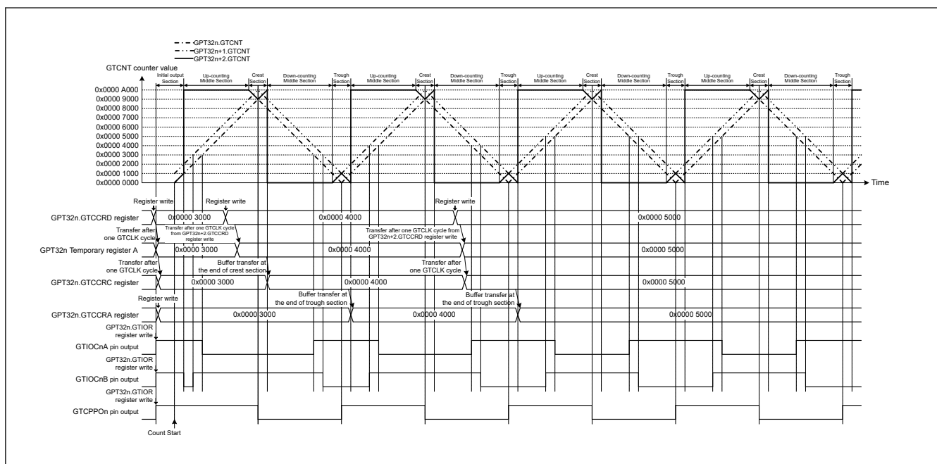
Figure 23.47 Example of Complementary PWM Mode 2 Operation (GTIOCnA pin = High / GTIOCnB pin = High as initial output, GTIOCnA pin = Low / GTIOCnB pin = High at GTCCRA register compare match during up-counting, GTIOCnA pin = High / GTIOCnB pin = Low at GTCCRA register compare match during down-counting, the dead time value is 0x0000 1000 and updating GTCCRD register in middle section) (n = 4, 7)
