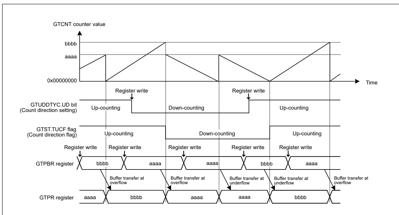
Figure 23.81 Example of a count direction changing function operation during buffer operation
