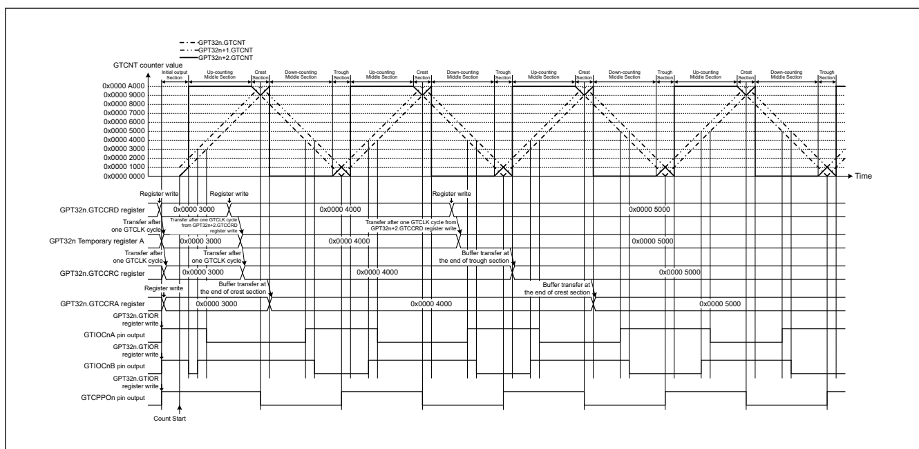
Figure 23.45 Example of Complementary PWM Mode 1 Operation (GTIOCnA pin = High / GTIOCnB pin = High as initial output, GTIOCnA pin = Low / GTIOCnB pin = High at GTCCRA register compare match during up-counting, GTIOCnA pin = High / GTIOCnB pin = Low at GTCCRA register compare match during down-counting, the dead time value is 0x0000 1000 and updating GTCCRD register in middle section) (n = 4, 7)
