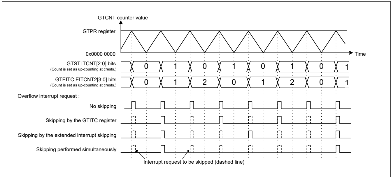
Figure 23.136 Example of Interrupt Skipping Operation (Skipping by the GTITC Register: Counting crests, Extended Interrupt Skipping: EIVTC1[1:0] bits = 00b, EIVTC2[1:0] bits = 01b, EITLV[2:0] bits = 010b)
