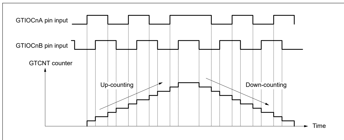
Figure 23.109 Example of phase counting mode 1
