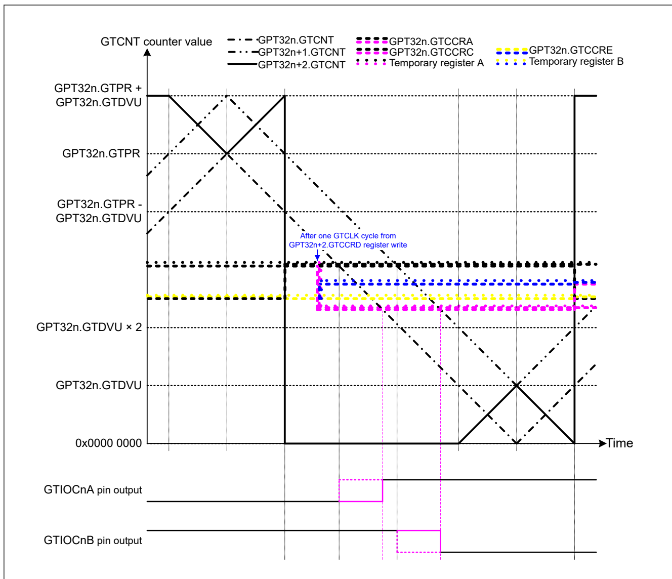
Figure 23.75 Example of Complementary PWM Mode 4 Double Buffer Operation (Down-Counting Middle Section) (Complementary PWM mode 4 double buffer operation, GTIOCN A pin = Low / GTIOCN B pin = High at GTCCRA register compare match during up-counting, GTIOCN A pin = High / GTIOCN B pin = Low at GTCCRA register compare match during down-counting, when a value smaller than the GPT32n.GTCNT value is written to GTCCRD register before down-counting compare match) (n = 4, 7)
