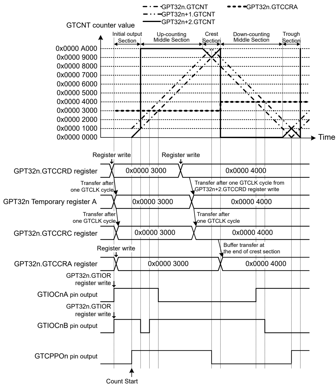
Figure 23.65 Example of Complementary PWM Mode Initial Output Operation (Complementary PWM mode 1 operation, GTIOCnA pin = Low / GTIOCnB pin = High at GTCCRA register compare match during up-counting, GTIOCnA pin = High / GTIOCnB pin = Low at GTCCRA register compare match during down-counting, the dead time value is 0x0000 1000, in the case that the initial GTCCRA register value is larger than the dead time value) (n = 4, 7)
