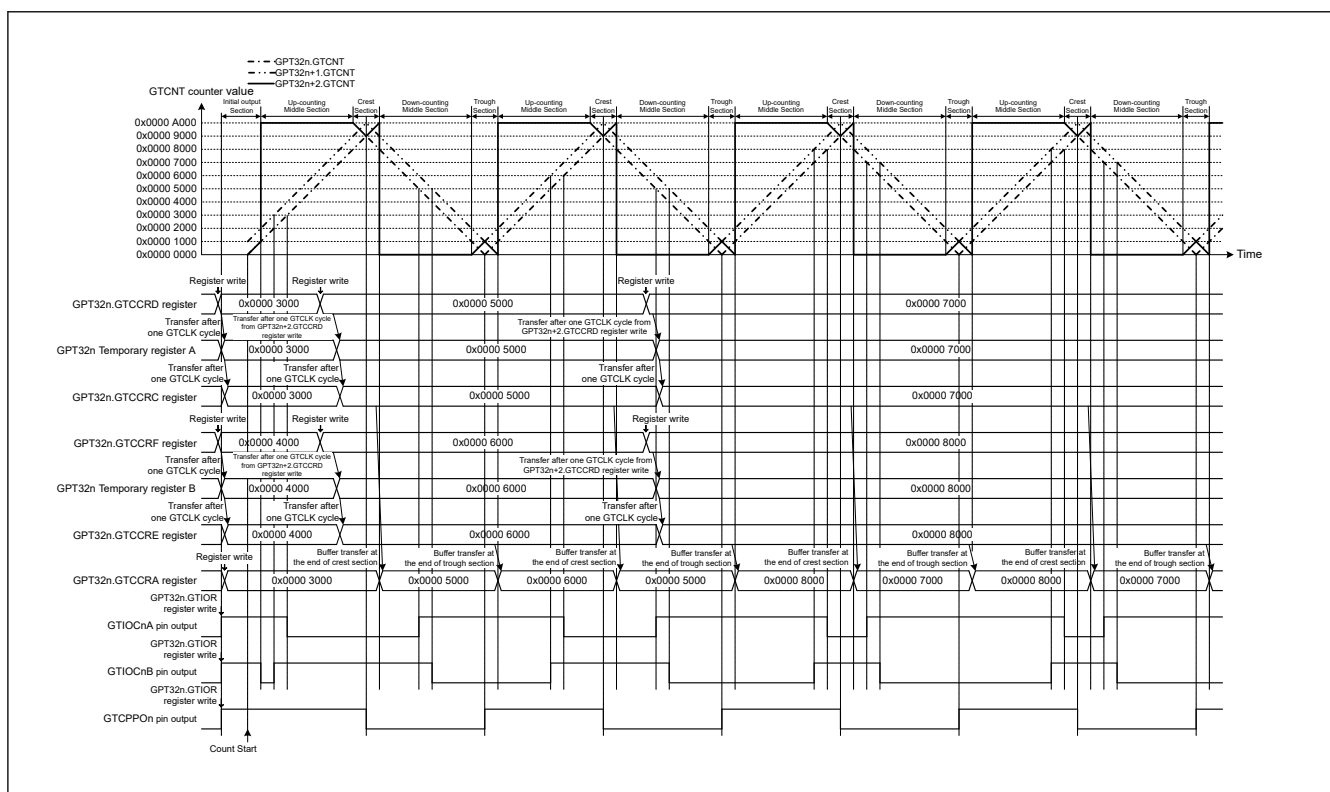
Figure 23.51 Example of Complementary PWM Mode 3 Operation (Double buffer operation, GTIOcNA pin = High / GTIOcNB pin = High as initial output, GTIOcNA pin = Low / GTIOcNB pin = High at GTCCRA register compare match during up-counting, GTIOcNA pin = High / GTIOcNB pin = Low at GTCCRA register compare match during down-counting, the dead time value is 0x0000 1000 and updating GTCRD register in middle section) (n = 4, 7)
