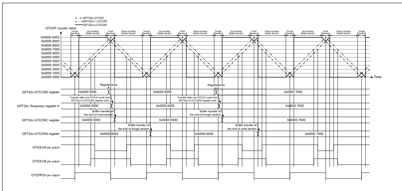
Figure 23.50 Example of Complementary PWM Mode 3 Operation (Single buffer operation, GTIOcNA pin = Low / GTIOcNB pin = High at GTCCRA register compare match during up-counting, GTIOcNA pin = High / GTIOcNB pin = Low at GTCCRA register compare match during down-counting, the dead time value is 0x0000 1000 and updating GTCRD register in crest and trough sections) (n = 4, 7)
