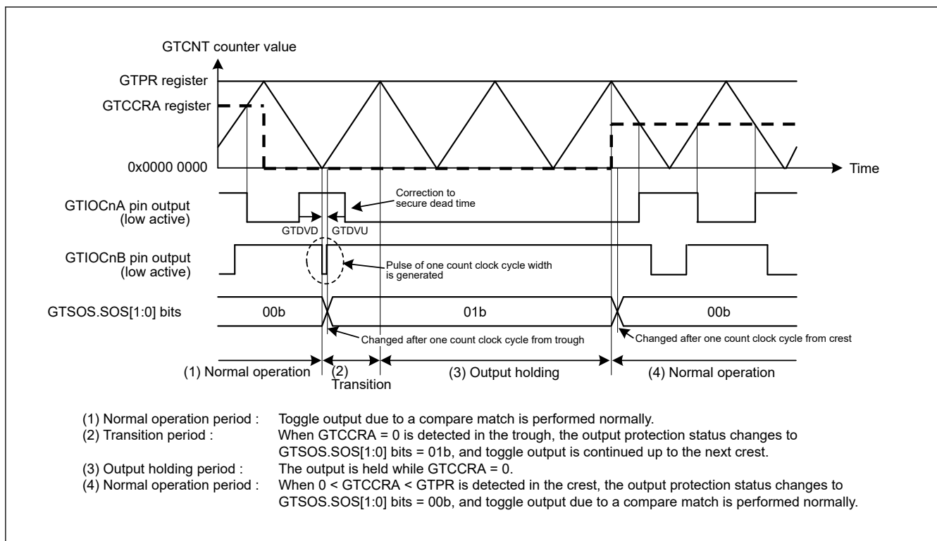
Figure 23.165 Example of Output Protection Function Operation When the GTCCRA is Set to 0x0000 0000 during Buffer Transfer at Crests (Restored to 0 < GTCCRA < GTPR during Buffer Transfer at Crests, Active Level: Low) (n = 0 to 13)
