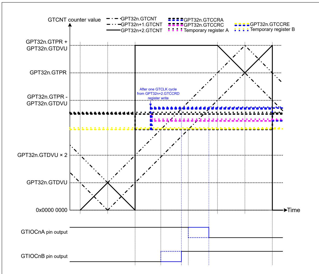
Figure 23.73 Example of Complementary PWM Mode 4 Double Buffer Operation (Up-Counting Middle Section) (Complementary PWM mode 4 double buffer operation, GTIOCnA pin = Low / GTIOCnB pin = High at GTCRA register compare match during up-counting, GTIOCnA pin = High / GTIOCnB pin = Low at GTCRA register compare match during down-counting, when a value larger than the GPT32n+1.GTCNT value is written to GTCCRF register before up-counting compare match) (n = 4, 7)
