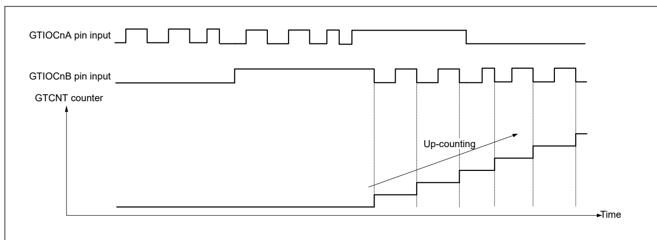
Figure 23.118 Example of phase counting mode 5 (B)
