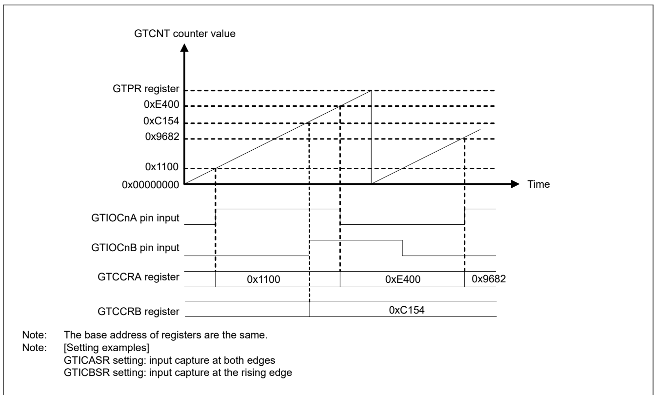
Figure 23.13 Example of input capture operation
